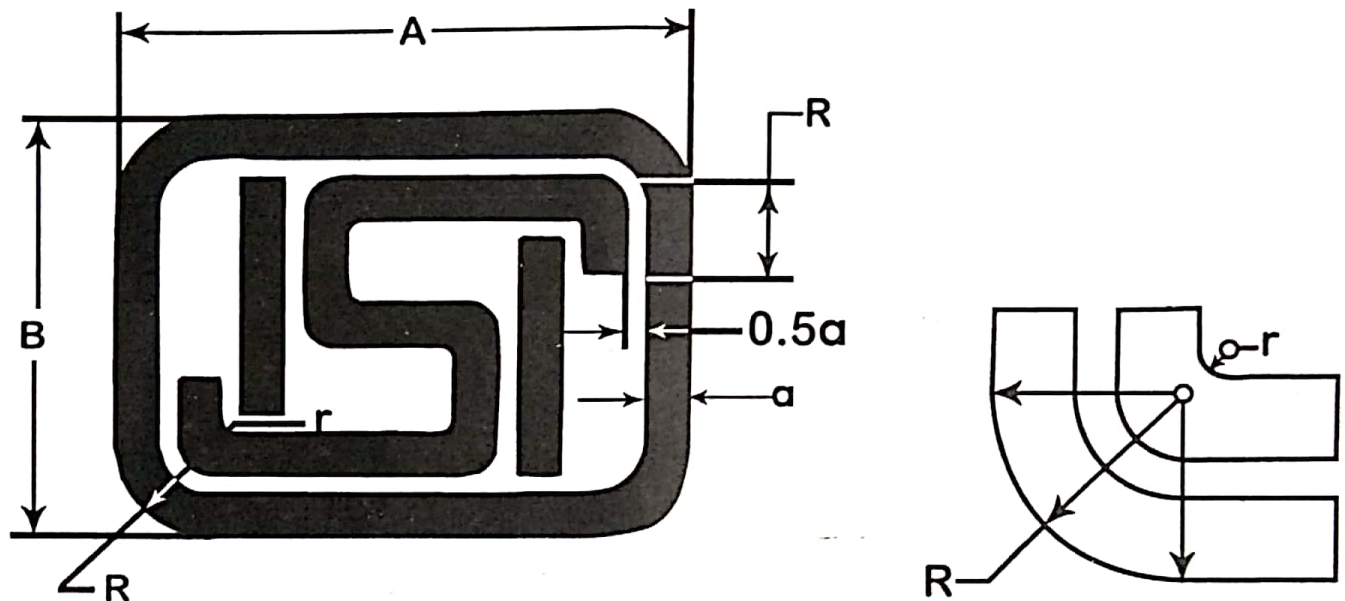
FIG. 1 MONOGRAM FOR STANDARD MARK
